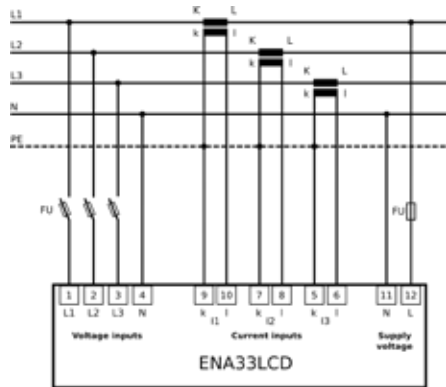
3-ph connection grid TN-C-S (TN-C)
